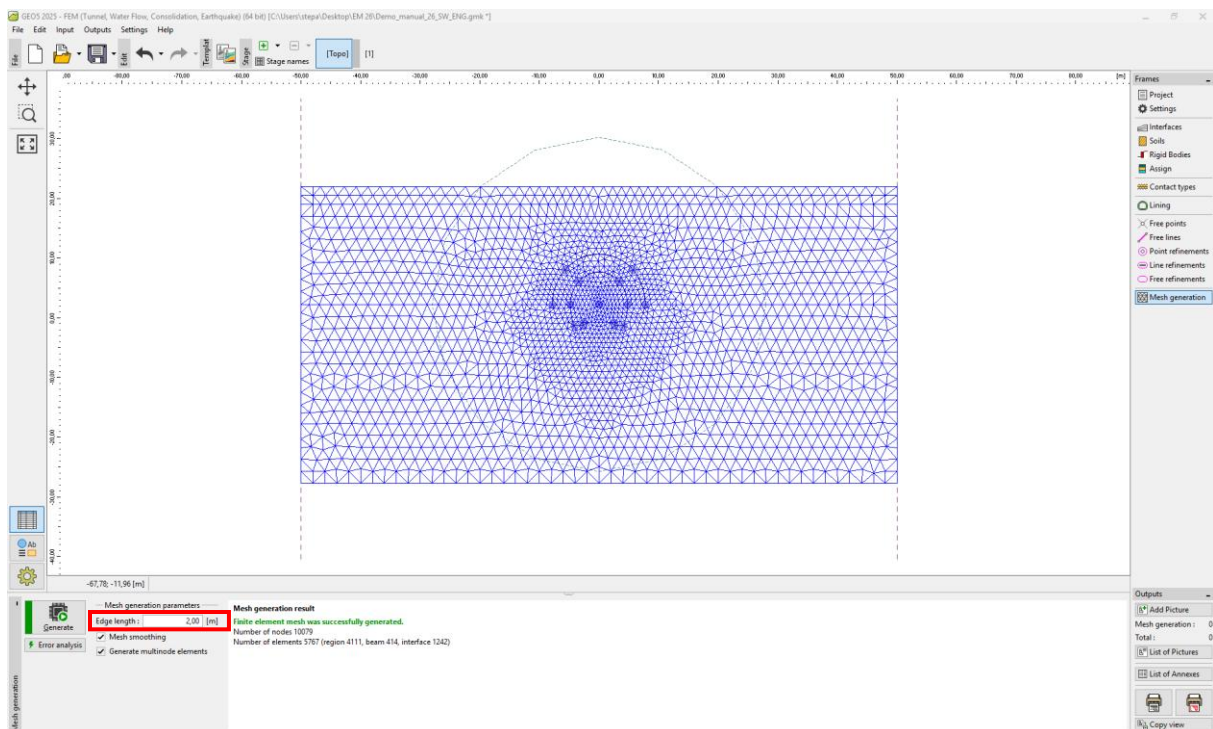
“Mesh generation” frame– Refinement of points near excavation region (length 0.5 m)
