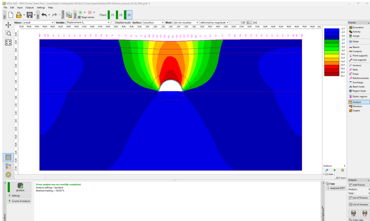
“Analysis” frame– Construction stage 3 (vertical displacement d_z with settlement trough)
