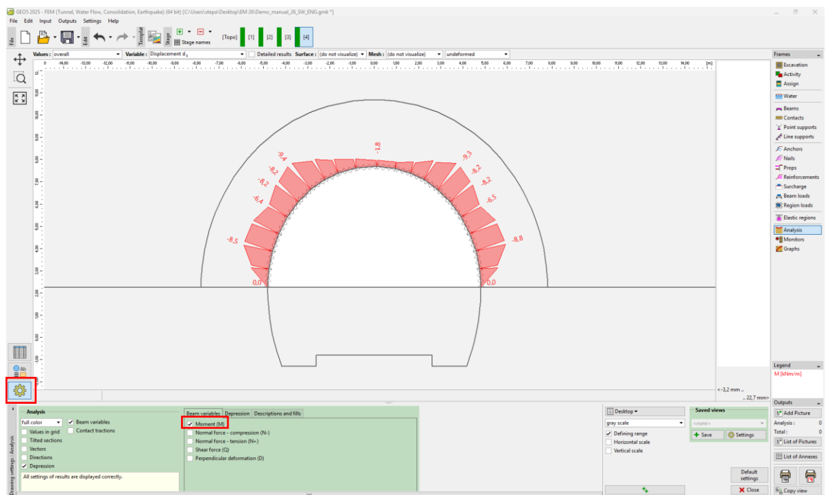
“Analysis” frame – Construction stage 4 (bending moment M [kNm/m])
