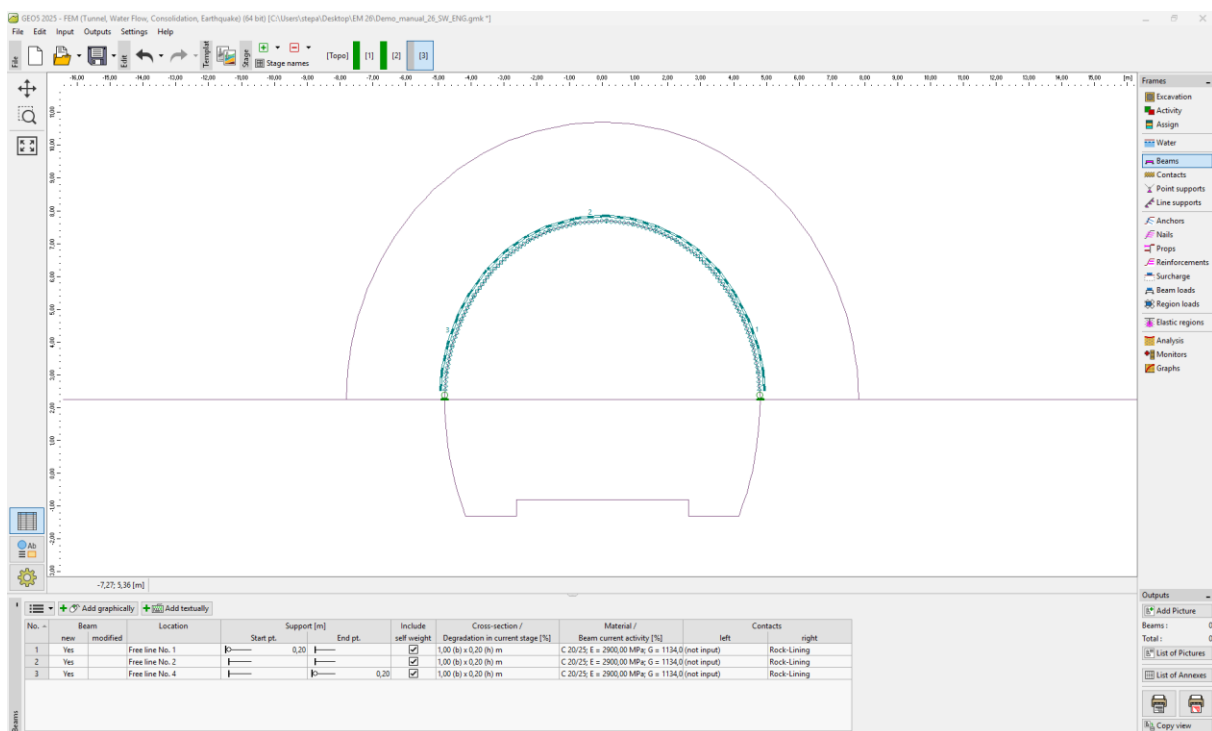
Input of primary lining of top heading with new beams – Construction stage 3 (immature concrete)
