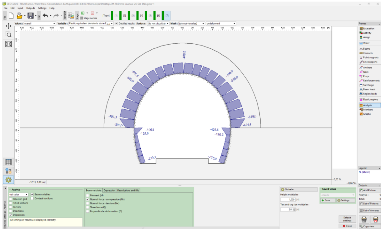
“Analysis” frame – Construction stage 7 (normal force – compression N^- [kN/m])
