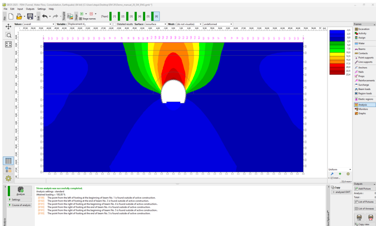
“Analysis” frame – Construction stage 6 (vertical displacement d_z with settlement trough)
