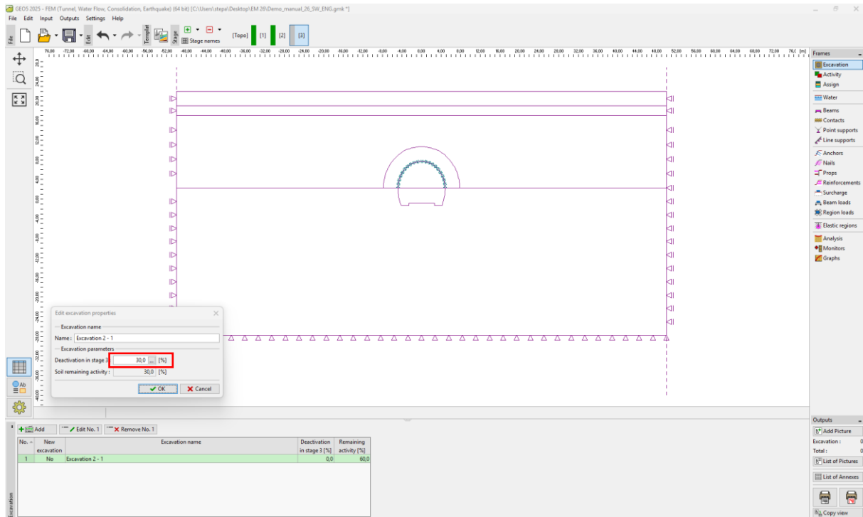
“Edit excavation properties” dialogue window – Construction stage 3
