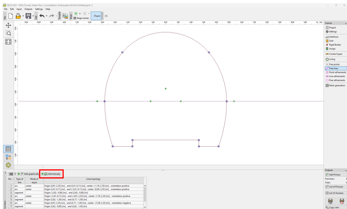
“Lining” module – FEM – Free lines of excavation (with horizontal sequencing)
