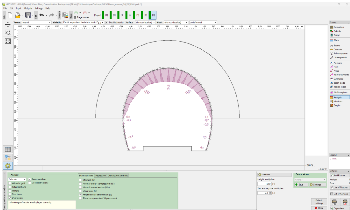
“Analysis” frame – Construction stage 7 (perpendicular deformation)
