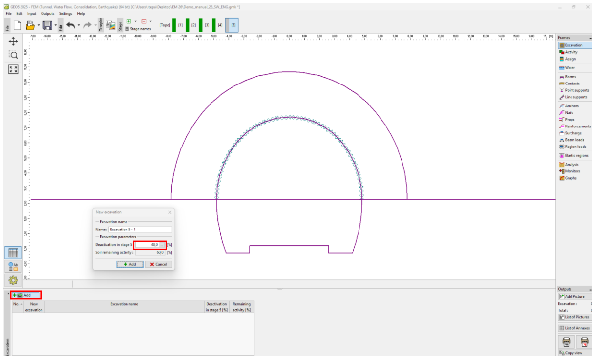
“New excavation” dialogue window – Construction stage 5
