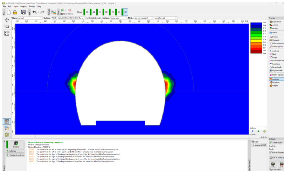
“Analysis” frame – Construction stage 7 (equivalent plastic strain \varepsilon_{eq.pl.} )
