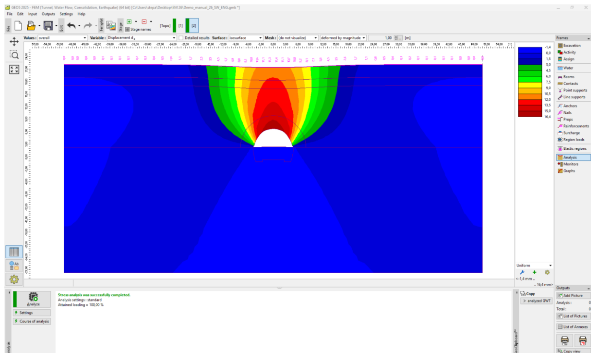
“Analysis” frame – Construction stage 2 (vertical displacement d_z with settlement trough)
