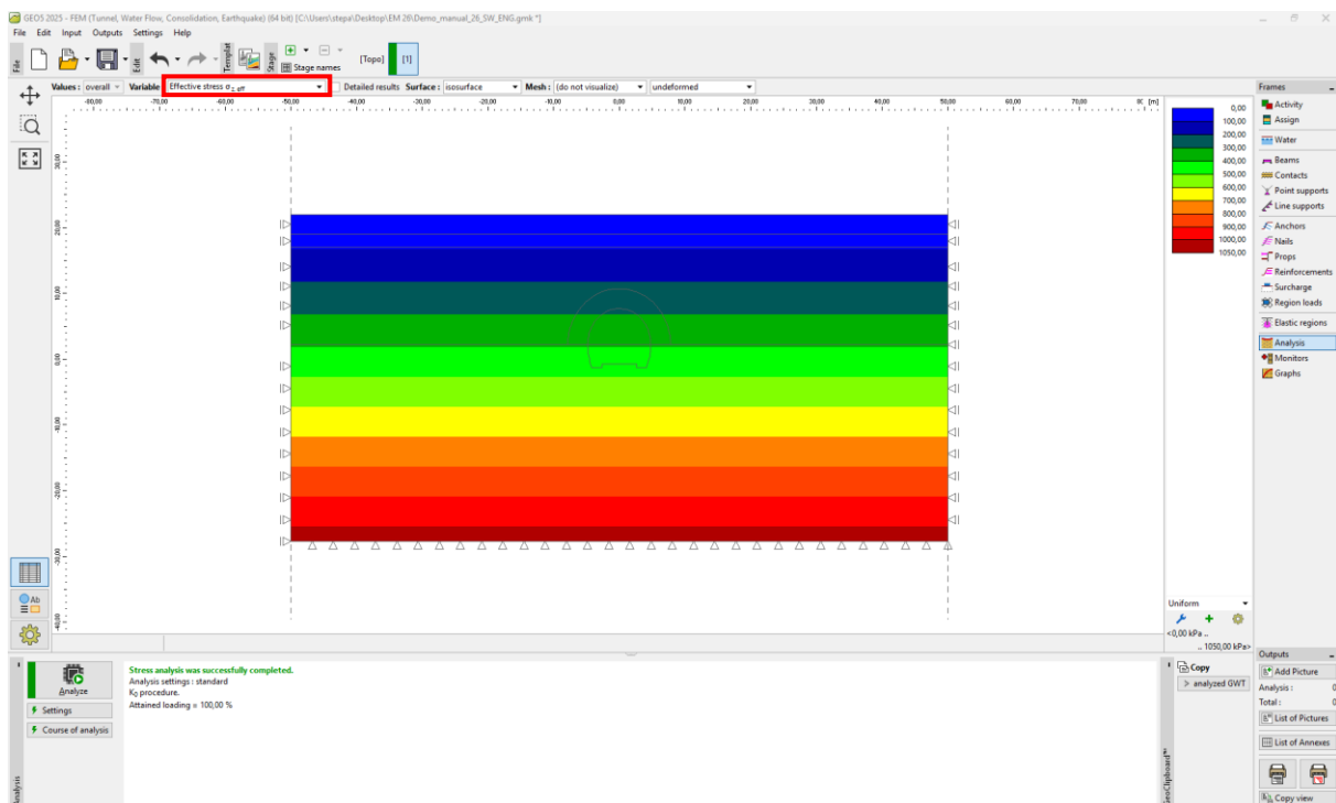
“Analysis” frame– Construction stage 1 (primary geostatic stress \sigma_{z,eff} )
