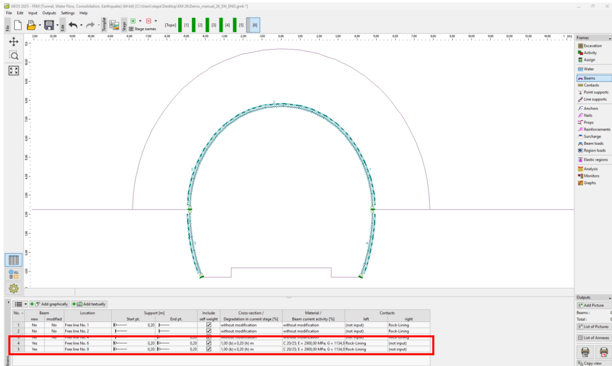
Input of primary lining of tunnel bench with new beams – Constr. stage 6 (immature concrete)
