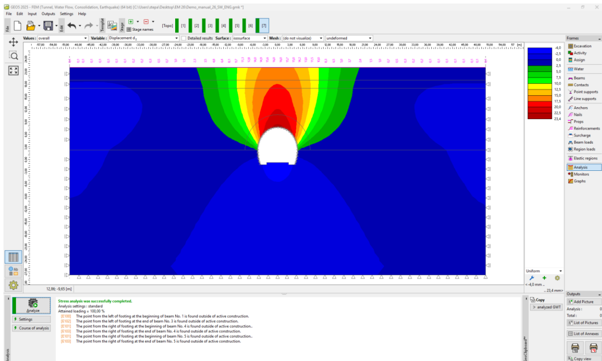
“Analysis” frame – Construction stage 7 (vertical displacement d_z with settlement trough)
