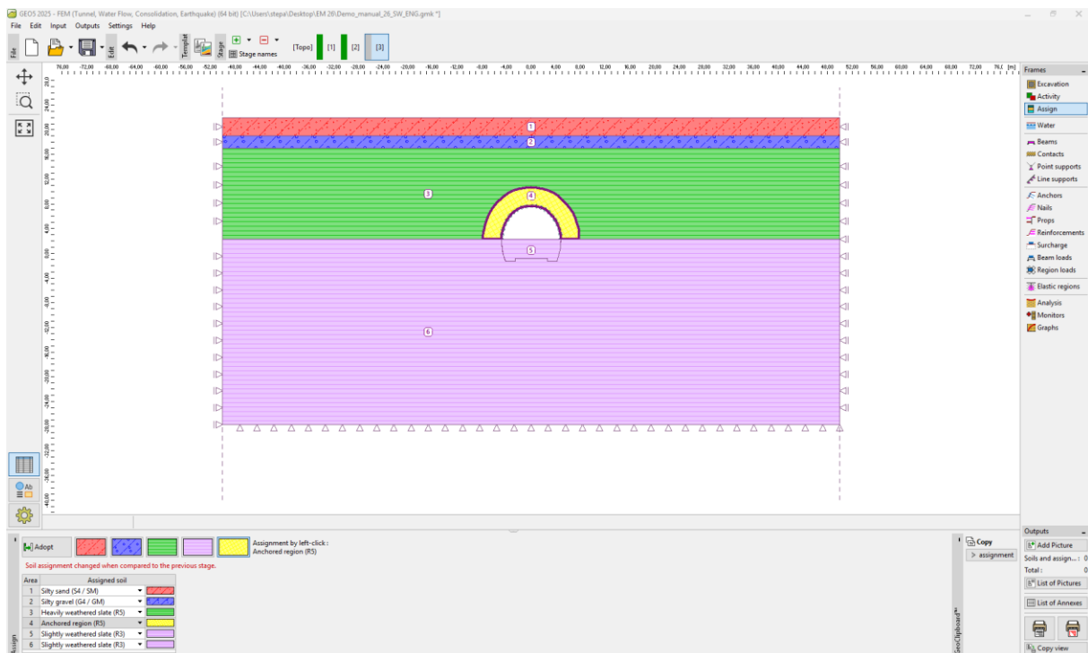
“Assign” frame – Constr. stage 3 (region anchored with hydraulically expanded rockbolts)
