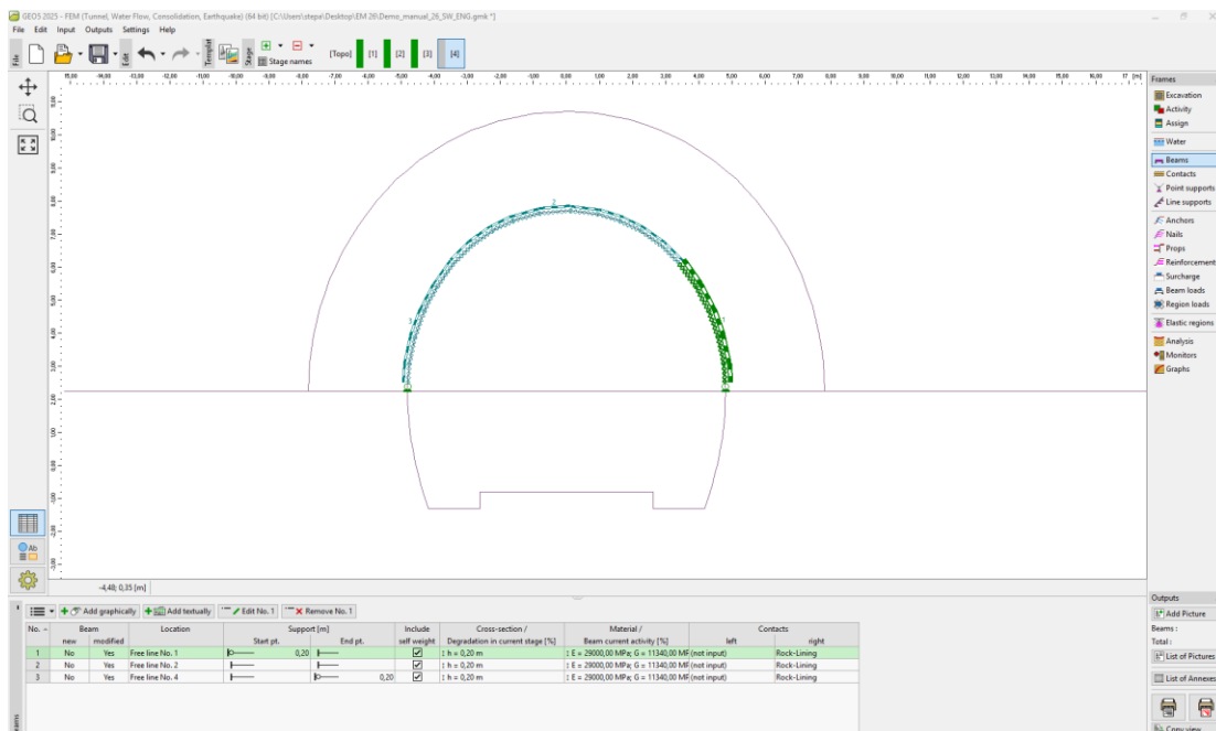
Modify properties of primary lining (top heading) – Construction stage 4 (mature sprayed concrete)
