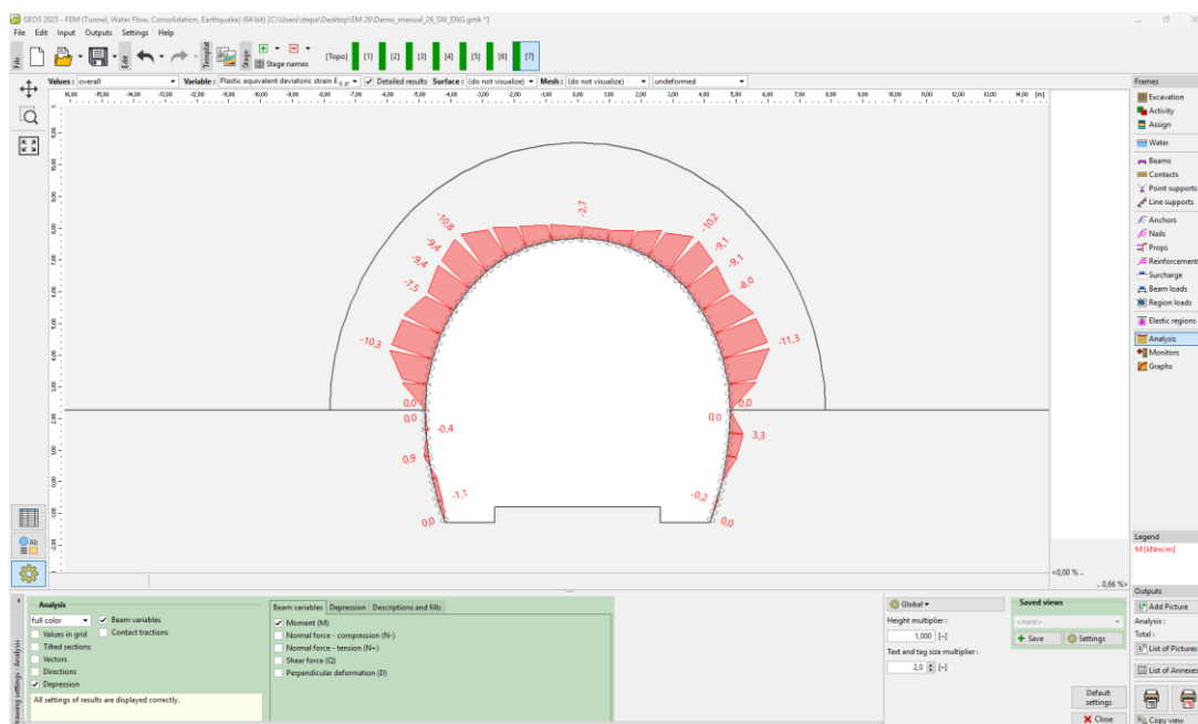
“Analysis” frame – Construction stage 7 (bending moment M [kNm/m])
